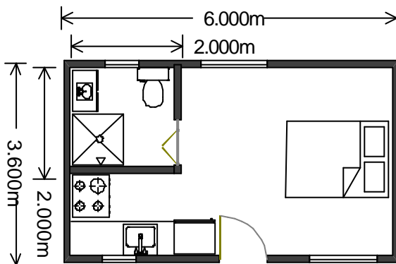
6 x 3.6 One Bedroom
